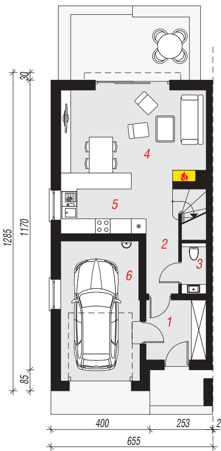
PARTER
