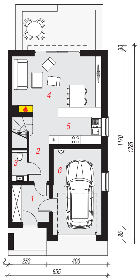
PARTER
