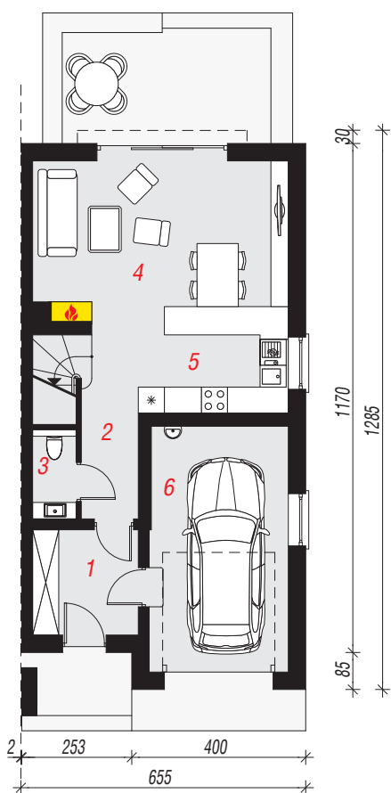
PARTER
