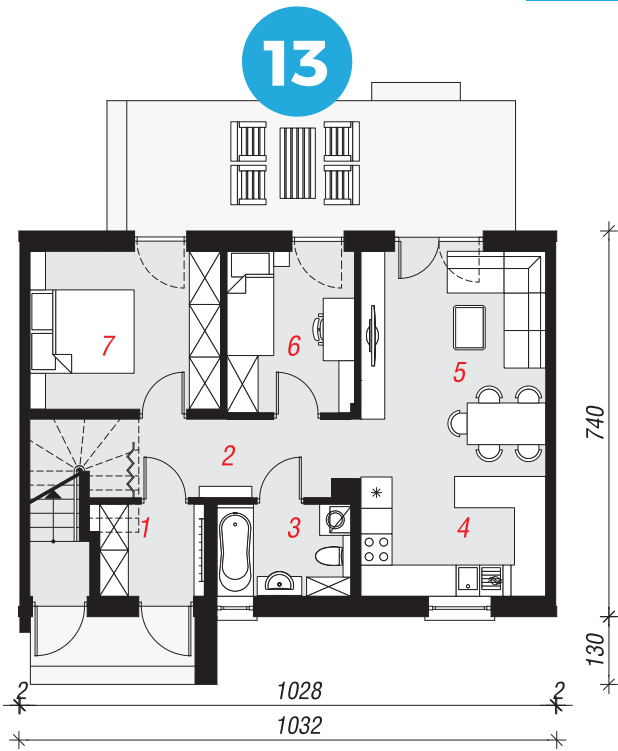
PARTER
